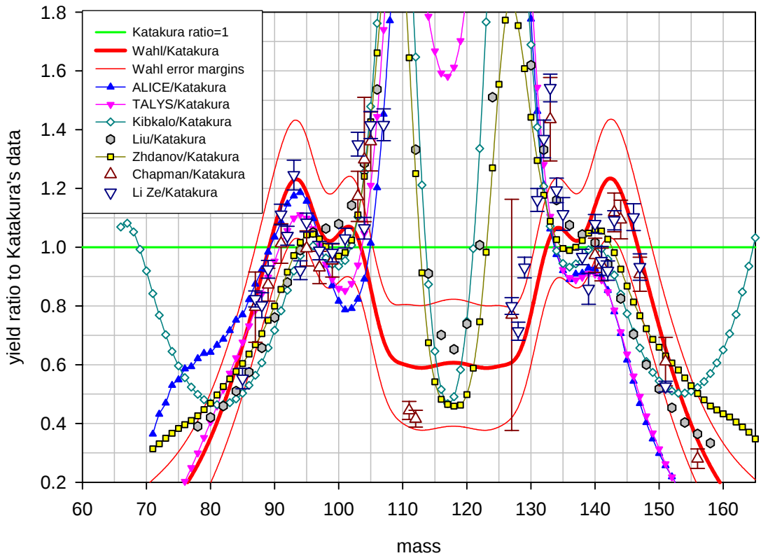
Benchmark A: ^{238}\text{U} at 7.0-8.3 MeV, post neutron emission yield ratios to Katakura's results lower graph is partial plot with high values omitted.
